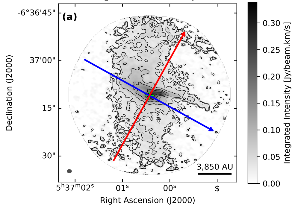
H 2 CO Moment 0 Map
