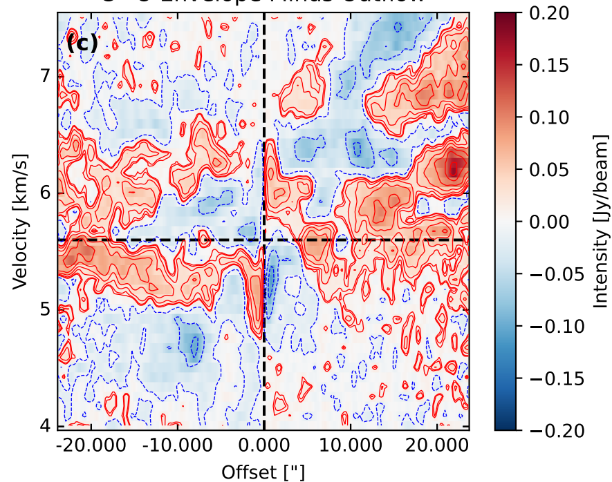
C 18 O Envelope Minus Outflow
