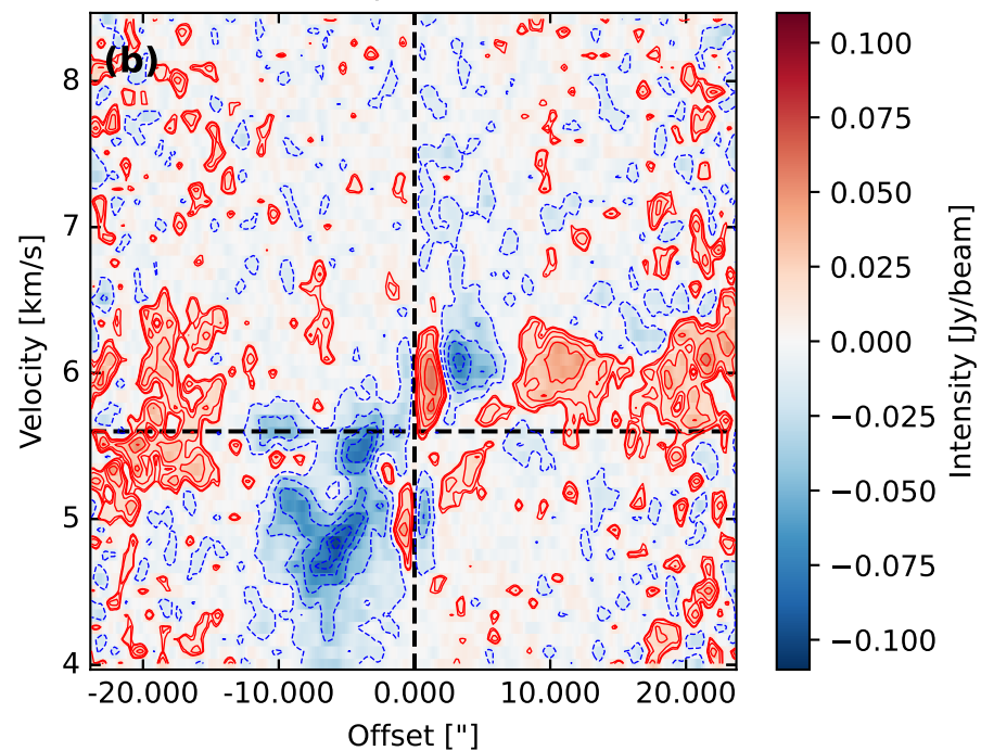
C 18 O Envelope Minus Outflow
